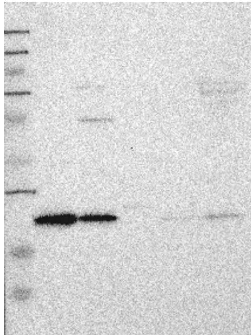
WB. Supportive (Band of predicted size in kDa (+/-20%) with additional bands present)
